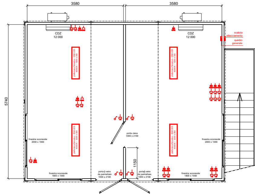
PLANIMETRIA PIANO TERRA
