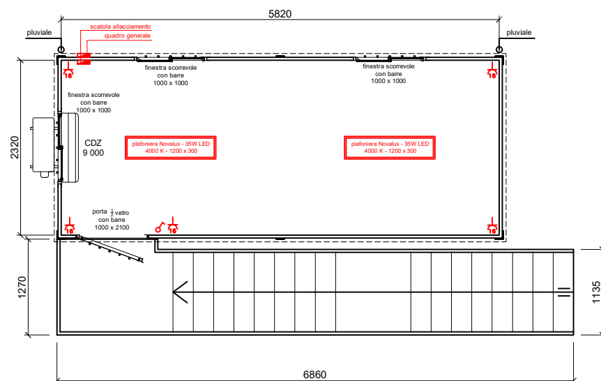
PLANIMETRIA PIANO TERRA
