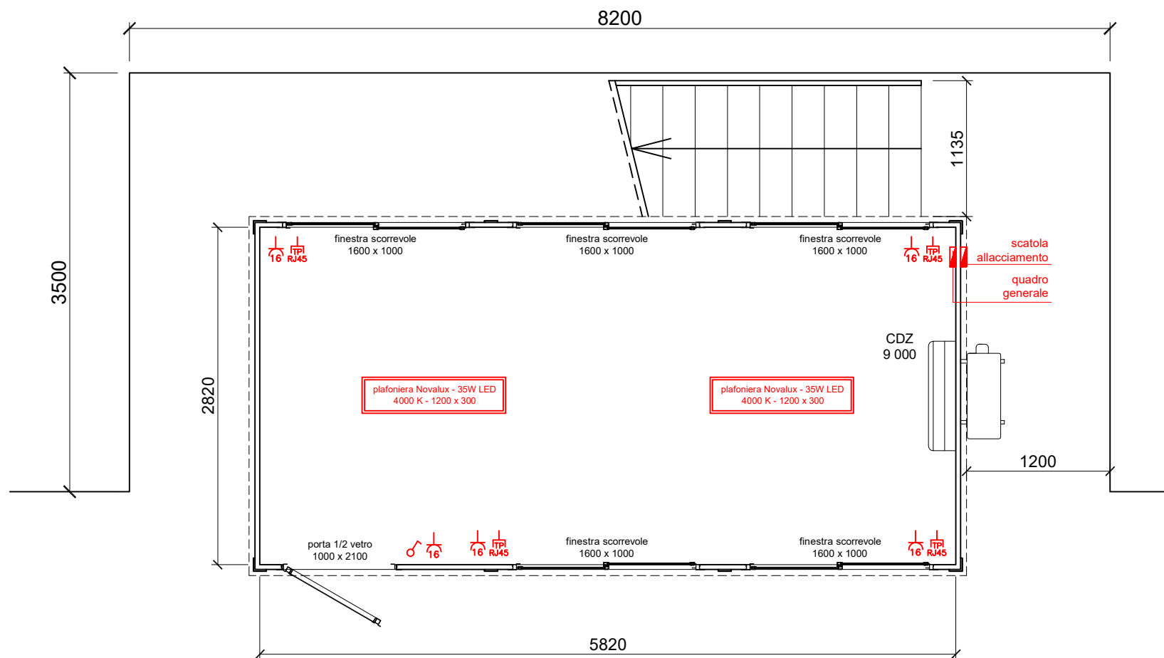
PIANO TERRA
