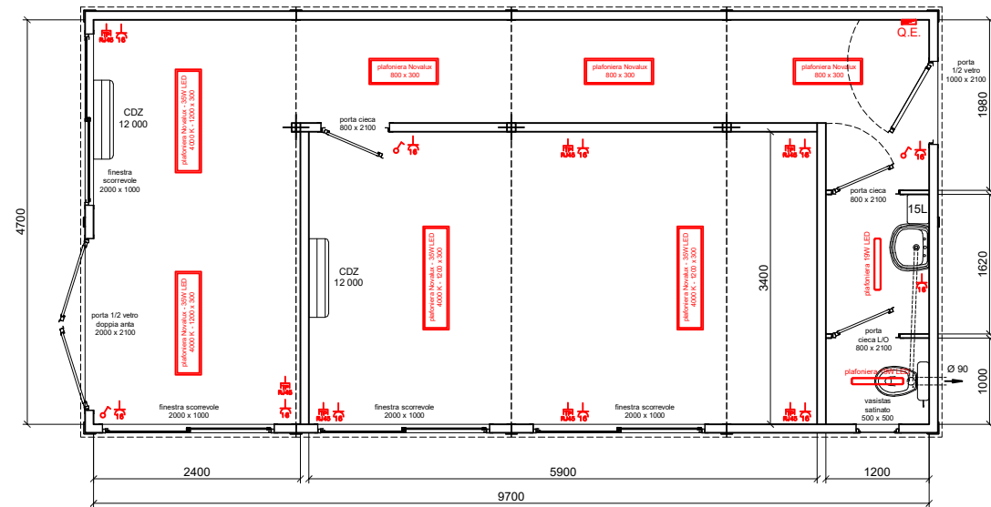
PIANO TERRA
